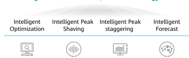
Figure 16: Intelligence values
