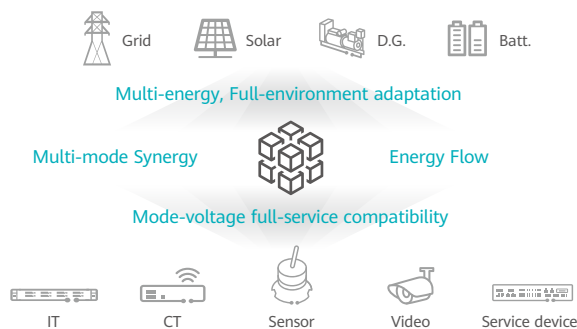
Figure 20: Multi-mode coordination
