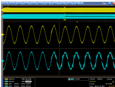
Figure 47 Chengde waveform (36th- and 38th-order)
