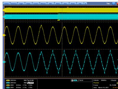
Figure 42 Spike wave
