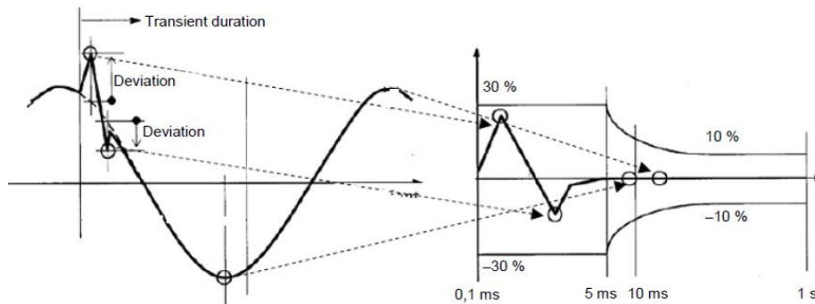
Figure 55 Criteria for UPS output dynamic response
