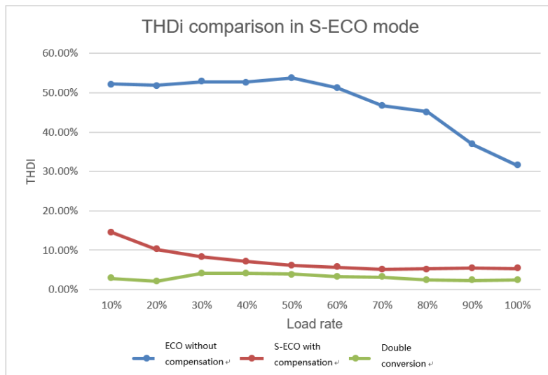
Figure 53 Input THDi comparison for harmonic compensation in S-ECO mode
