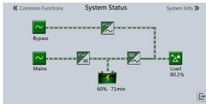
Figure 24 Power flow in S-ECO mode (without harmonic compensation)
