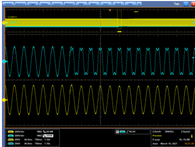
Figure 38 Triple harmonic
