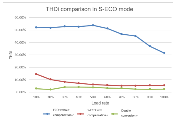
Figure 53 THDi comparison for harmonic compensation in S-ECO mode
