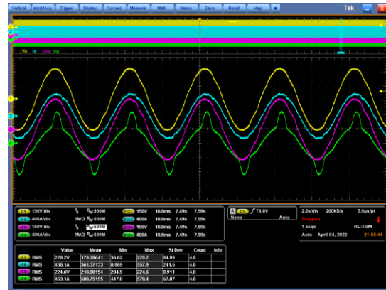
Figure 51 After compensation
