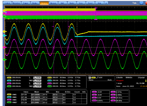
Figure 54 Output dynamic response verification
