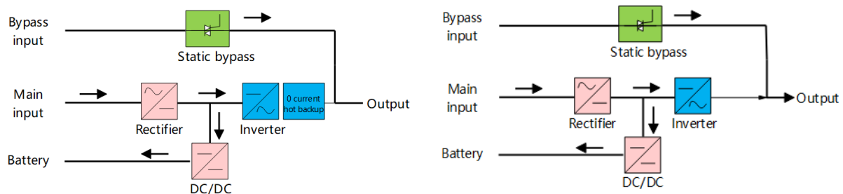
Figure 15 Zero-current hot backup (left) vs. Low-current hot backup (right)
