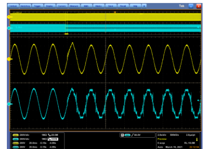
Figure 46 Chengde waveform (37th- and 39th-order)
