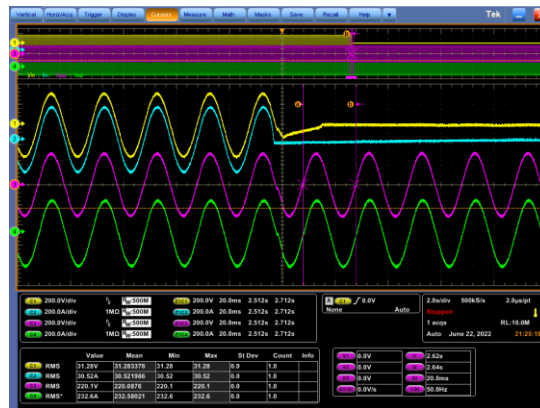
Figure 35 Yellow: bypass input voltage; blue: bypass input current; purple: system output voltage; green: system output current
