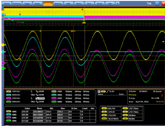
Figure 27 Switching upon overvoltage ( \geq 242 V)
