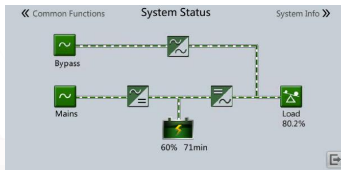
Figure 25 Power flow in S-ECO mode (with harmonic compensation)
