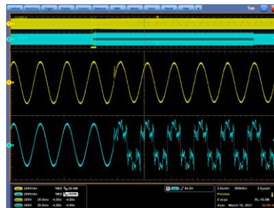
Figure 45 Steel mill waveform 2 (mainly 5th-, 7th-, and 11th-order harmonics)
