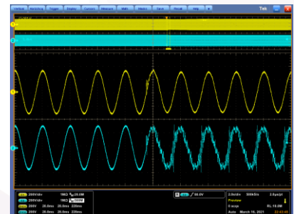
Figure 49 Steel mill waveform 3 (1.5 kHz square wave superimposed)
