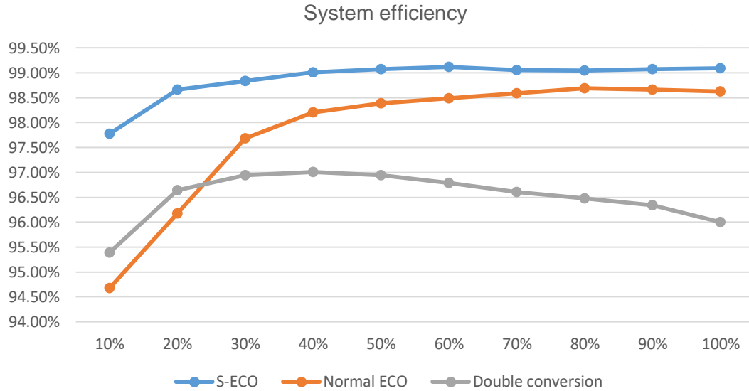
Figure 58 Efficiency curve in S-ECO mode
