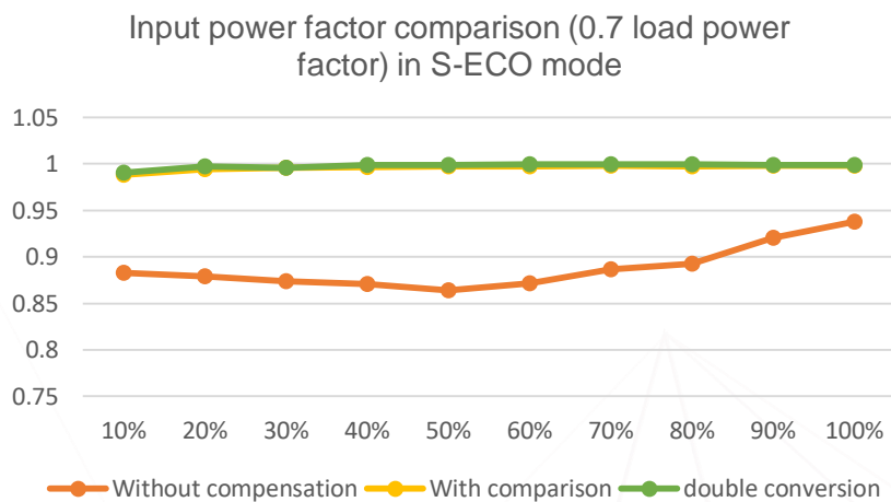
Figure 52 PF comparison for harmonic compensation in S-ECO mode
