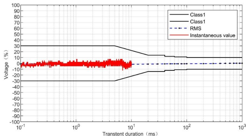
Figure 56 Test result of the dynamic output response of the UPS5000-H in S-ECO mode
