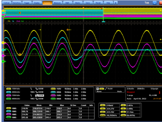
Figure 31 Switching upon overfrequency ( \geq 56 Hz)
