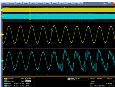
Figure 44 Mining plant waveform 3 (1 kHz 50 V square wave superimposed, mainly 2nd-, 20th-, and 40th-order harmonics)
