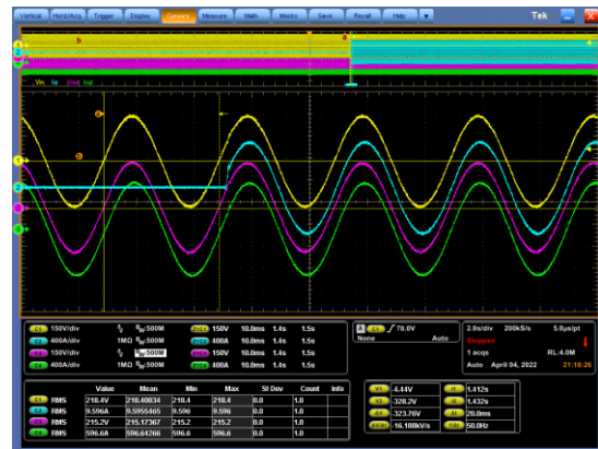
Figure 32 Recovery at normal frequency (50 Hz)
