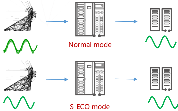
Figure 12 Recommended operating modes for different power grid quality
