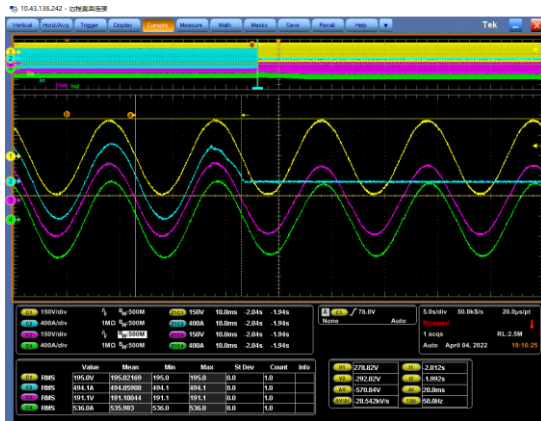
Figure 29 Switching upon undervoltage ( \leq 198 V)
