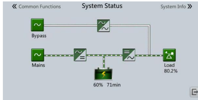
Figure 26 Power flow in S-ECO mode (transfers to online mode)
