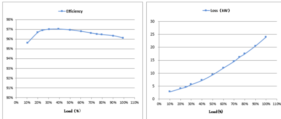
Figure 61 Report excerpt (efficiency test)
