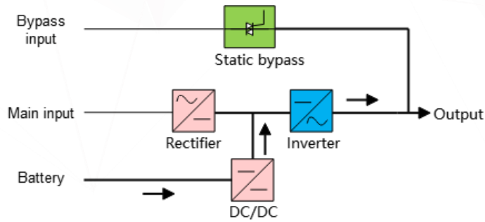
Figure 5 Online double-conversion mode (battery mode)
