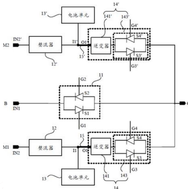
Figure 16 Patented diagram of the S-ECO technology
