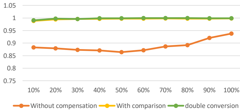
Figure 52 PF comparison for harmonic compensation in S-ECO mode
