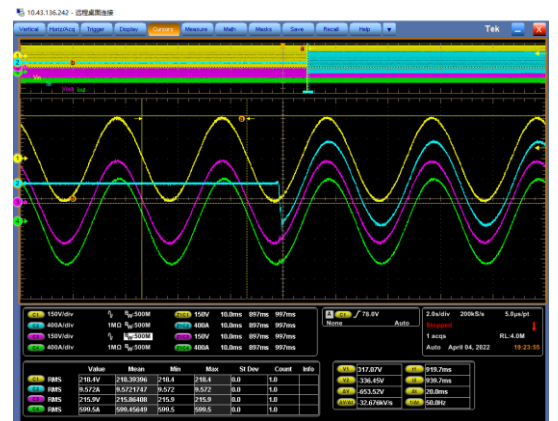
Figure 30 Recovery at normal voltage (220 V)
