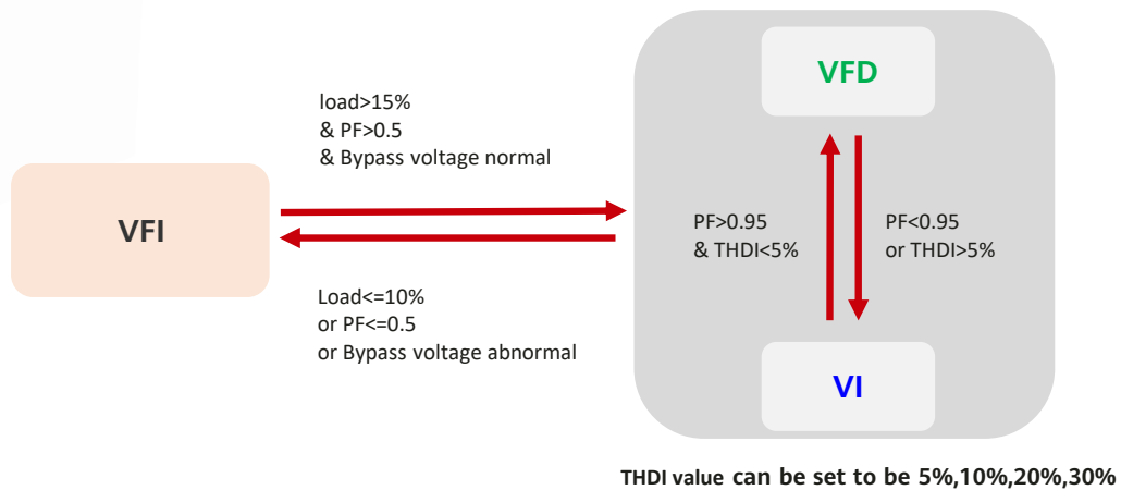
Figure 23 Status switching in S-ECO mode
