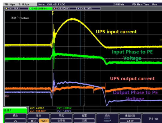
Figure 37 Common-mode 6 kV surge test waveform
