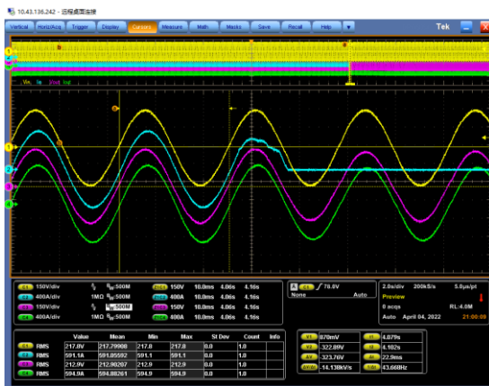
Figure 33 Switching upon underfrequency ( \leq 44 Hz)
