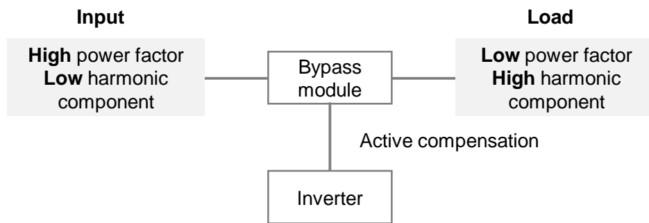
Figure 11 Active harmonic compensation
