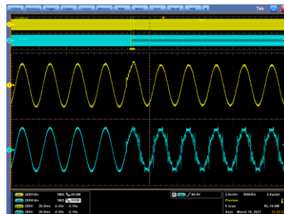
Figure 48 Anshan waveform (29th- and 31st-order)
