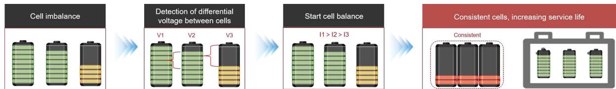
Figure 13 Battery balancing management process
